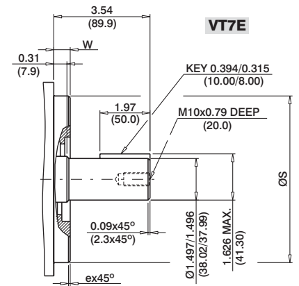
Shaft code 5 (Keyed ISO R775 - G38M)
