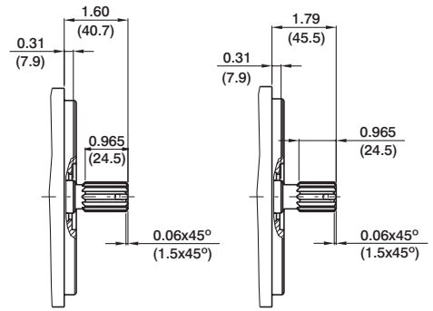
Shaft code 4 SAE BB splined shaft Class 1-J498b 16/32 dp. 15 teeth 30° pressure angle flat root side fit
