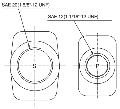
PORT CONNECTION 00
