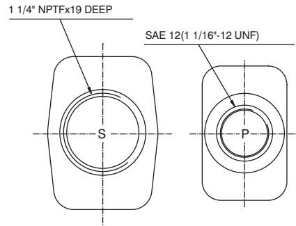
PORT CONNECTION 03
