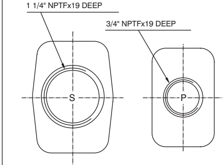
PORT CONNECTION 0X
