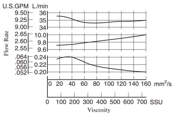
Metred Flow vs. Viscosity
