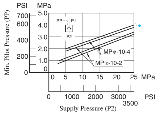
Min. Pilot Pressure
