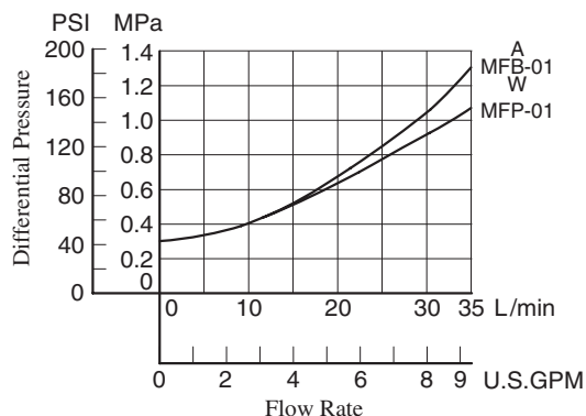
Min. Required Pressure Difference
