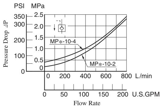
Pressure Drop for Free Flow
